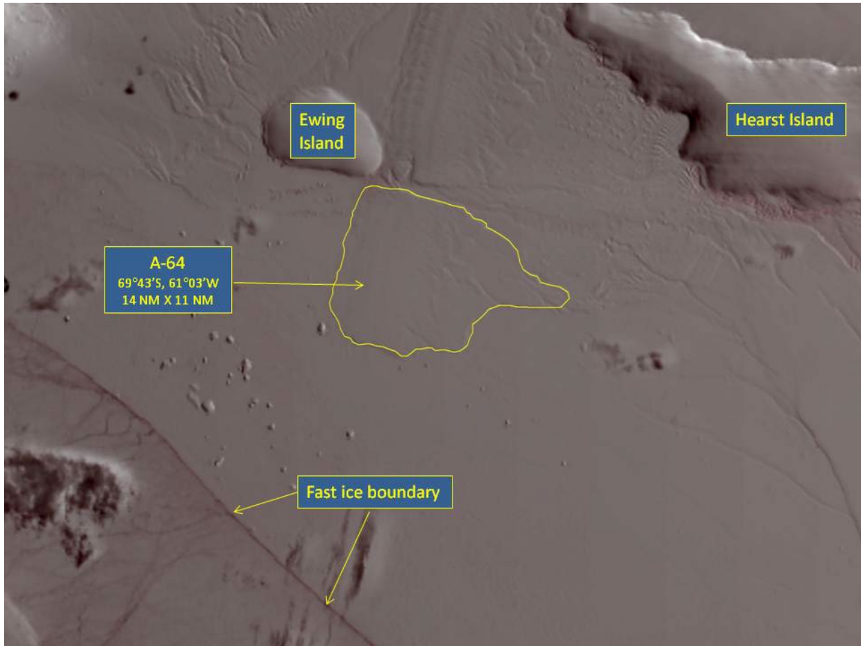
MODIS image of A-64, March 24, 2014
